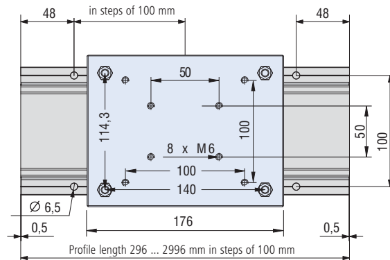
LFS-8-3 with trolley LW7
