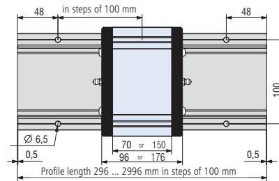
LFS-8-3 with aluminium slide WS 3/70 or WS 3
